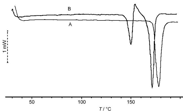
Figure 3. Thermal analysis (DSC) of form I (A) and II (B) crystals of rac -3.
