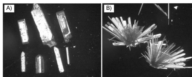
Figure 2. Photomicrographs of form I (A) and II (B) crystals of rac -3.
