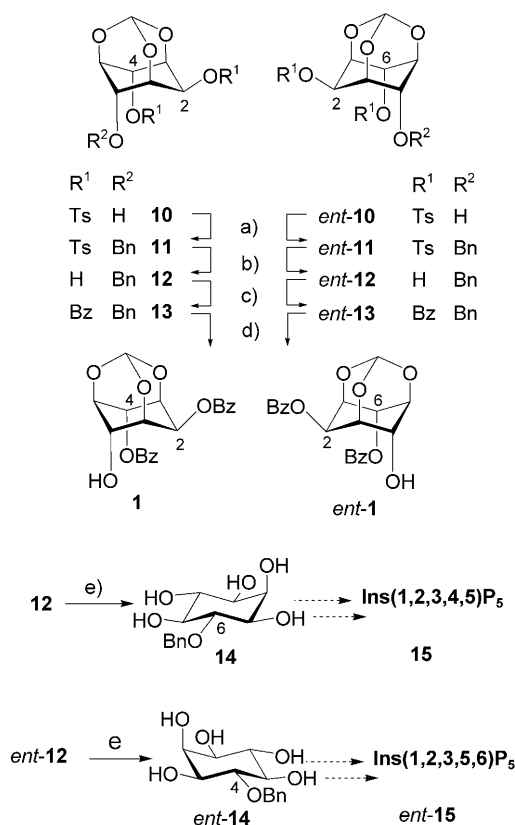
Scheme 2. Preparation of enantiomeric myo -inositol derivatives. a) DMF, BnBr, NaH, 0°C–RT, 30 min, 94–96%; b) NaOMe, MeOH, reflux, 12 h, 92–98%; c) pyridine, BzCl, RT, 20 h, 96–98%; d) ethyl acetate/methanol, Pd(OH) 2 /C, H 2 (55 psi), RT, 6 h, 94–96%; e) TFA/H 2 O (4:1 v/v), RT, 24 h, 84–87%. TFA = trifluoroacetic acid.
