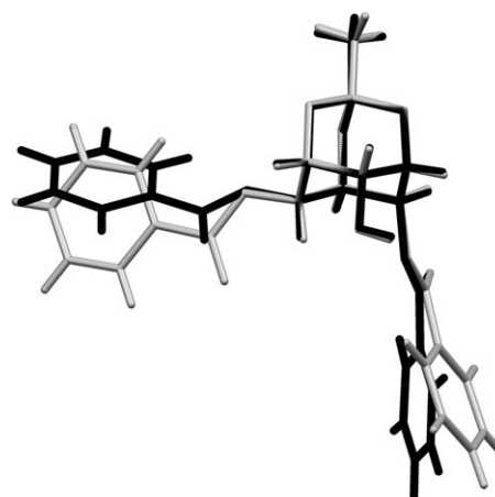
Figure 5. Overlap diagram of molecules present in crystals of form I (black) and II (light grey) of rac - 3 .
