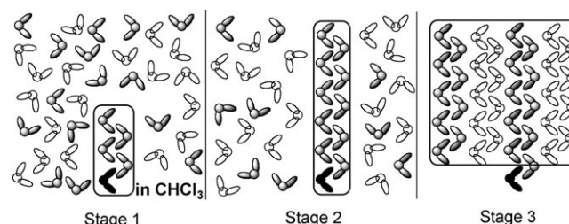
Figure 7. Stage 1: Nucleation of the form II crystal (of rac-3 ), with the aid of ent-1 (or 1 ), by the aggregation of molecules of rac-3 with the same relative configuration as ent-1 (or 1 ). This molecular assembly is suggested to be isostructural to that of the co-crystal rac-1-rac-3 . Stage 2: Growth of the helix along the screw axis, by assembly of molecules of rac-3 with the same configuration ( D or L ). Stage 3: Complementary helical assembly (helix constituted by plain molecules) of molecules of rac-3 leading to complete crystal formation and its stabilization. Filled molecules: 1 or ent-1 ; plain molecules: one of the enantiomers of rac-3 ; shaded molecules: enantiomer of rac-3 with a configuration opposite to that of the plain molecule.
