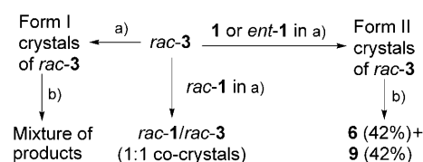
Scheme 3. Acyl-transfer reactions in crystals of rac - 3 . a) Chloroform/light petroleum; b) \text{Na}_2\text{CO}_3 , 115°C.
