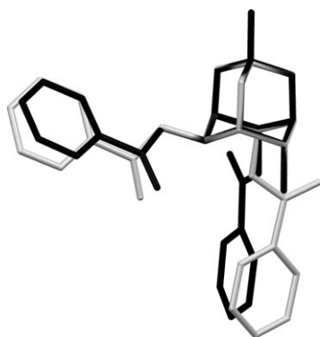
Figure 1. Overlap diagram of molecules present in crystals of ent -1 (light grey) and rac -3 (black).
