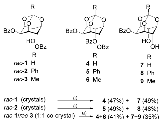
Scheme 1. Solid-state transesterification reactions in crystals of myo -inositol orthoester derivatives. a) Na 2 CO 3 , heat.
