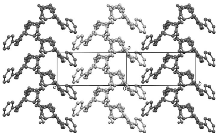
Figure 8. Helical assembly of molecules in crystals of ent - 1 viewed diagonal to the bc plane.
