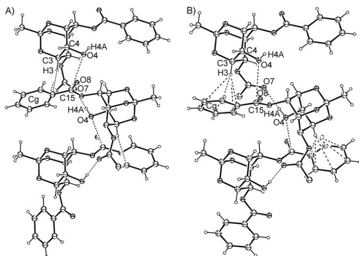
Figure 4. Comparison of El···Nu geometry and allied weak interactions in form I (A) and II (B) crystals of rac - 3 .
