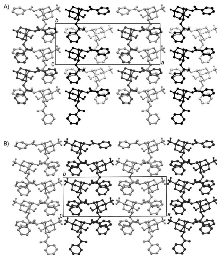
Figure 6. Comparison of the molecular organization in A) co-crystal rac-1-rac-3 and B) form II of rac-3 viewed down the c axis.
